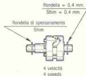
FIG. 28 Desmodromico Gear-box cam
