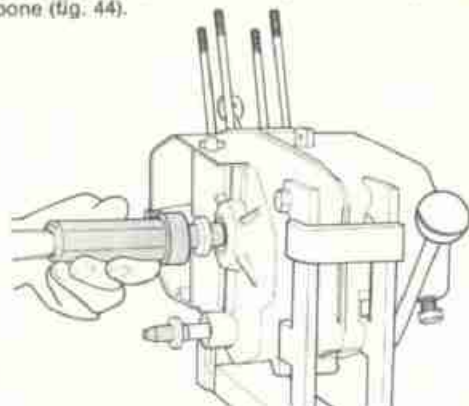
FIG. 44 Montaggio paraoli Oil seals assembly
